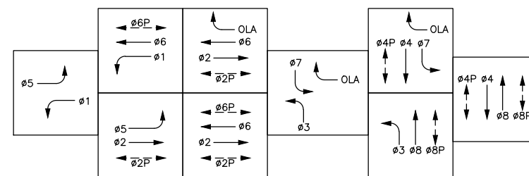
PHASE DIAGRAM
