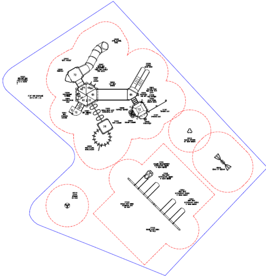
Plan View – Equipment Layout
