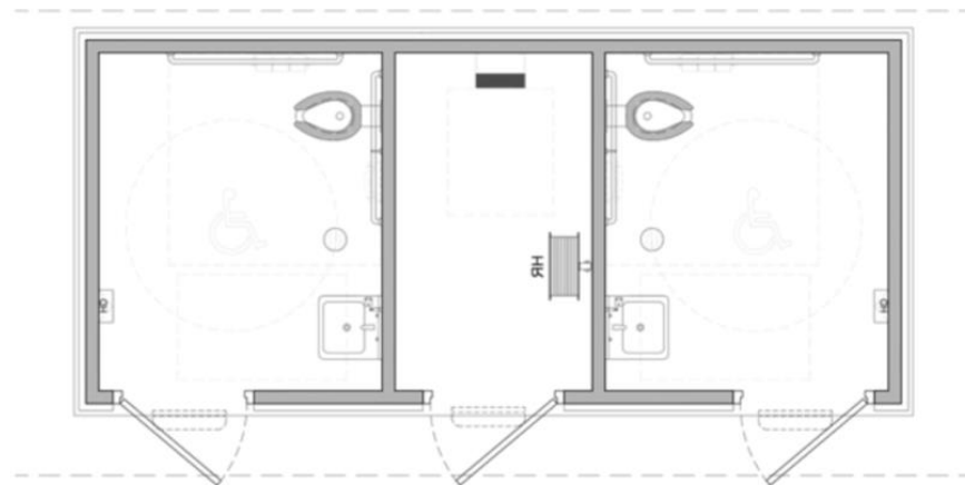
Restroom Layout
