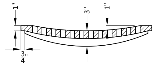
SECTION E-E
