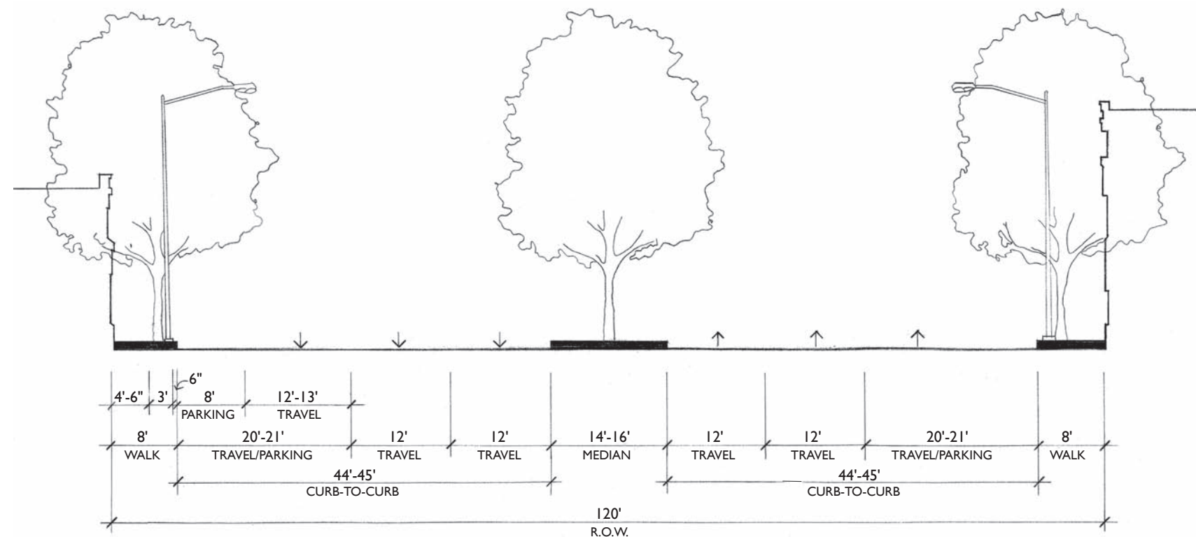
Figure 3.2: Urban 6-Lane
