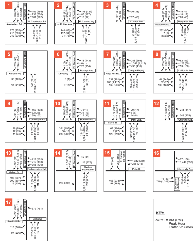
El Camino Real Schematic Design FUTURE PEAK HOUR TRAFFIC VOLUMES FIGURE 2
