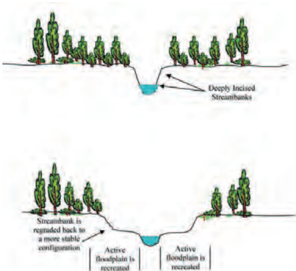
FIGURE 3: LAYING BACK A STREAMBANK TO INCREASE STABILITY
