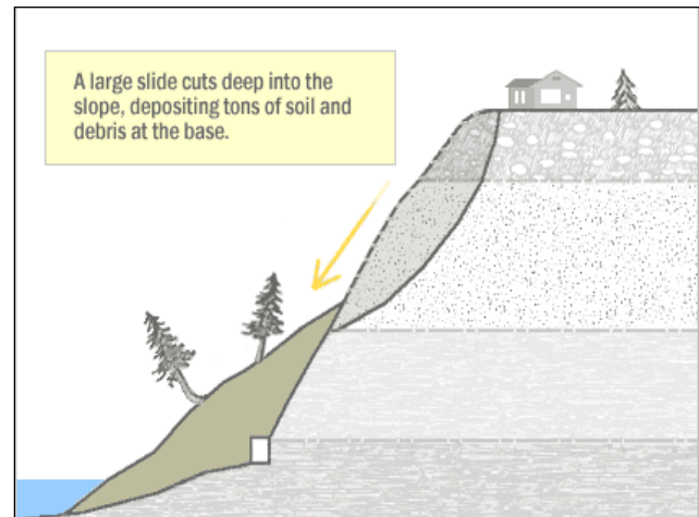
FIGURE 10-4. LARGE SLIDE
